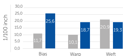
ELONGATION UNDER 20 LBS
