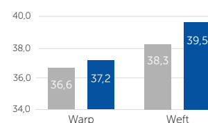
BREAKING STRENGTH (DaN/cm)
